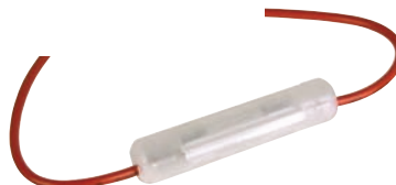
BF310 10A- 18AWG wire AGC/JMC fuses
