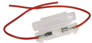
BF310 10A- 18AWG wire AGC/JMC fuses
