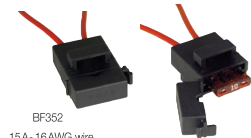
BF351 25A- 12AWG wire water resistant ATP/ATC/ATO fuses
