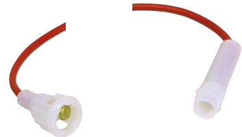
BF309 20A- 16AWG wire AGC/JMC fuses
